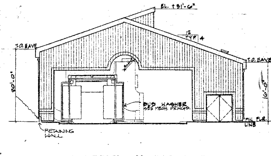
EAST ELEVATION 1/8" = 1'-0" - SEE WEST BLEV. FOR TYP. NOTES
