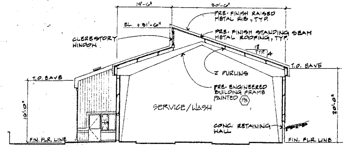
SOUTH ELEVATION 1/8" = 1'-0" - SEE NORTH BLEV. FOR TYP. NOTES
