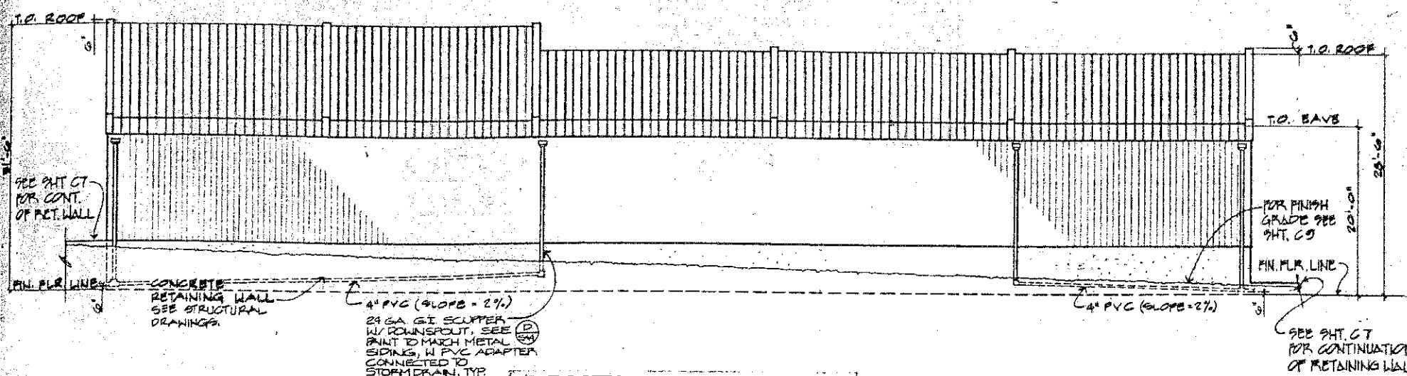
SOUTH ELEVATION 1/8" = 1'-0" - SEE NORTH BLEV. FOR TYP. NOTES
